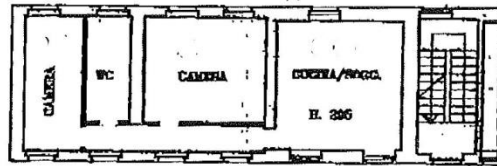
PIANO TERRA
